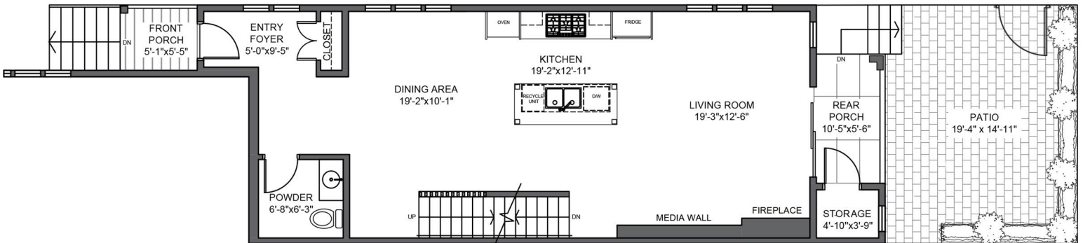
MAIN FLOOR Ceiling Height: 9'
